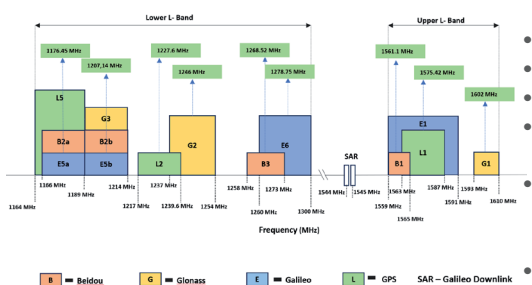
GNSS Frequencies in L Band
